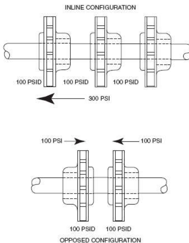
Figure 13-1 Impeller orientation.
