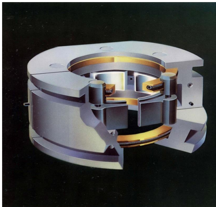
Δ Fig. 8 Multi-segment journal bearing with four tilting pads.
