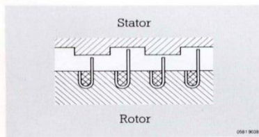
Δ Fig. 7 Labyrinth shaft seals.
