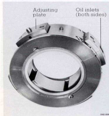
Δ Fig. 8 Multi-segment journal bearing with four tilting pads.
