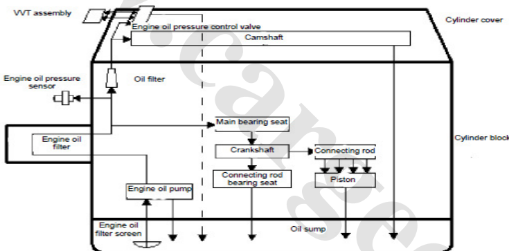
Lubrication system
