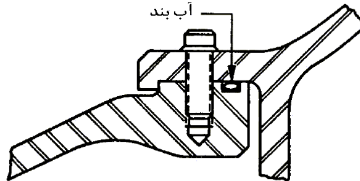
bolted-shear lip
