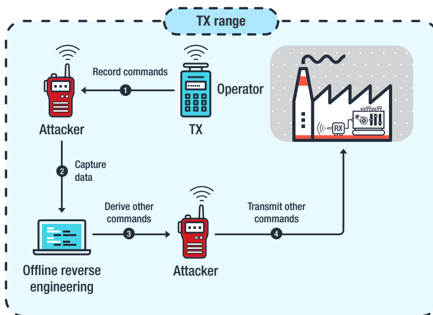
Figure 14. Conceptual representation of a command injection attack on an industrial radio remote controller
