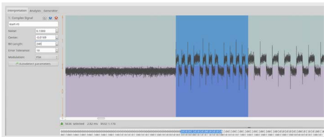
Figure 31. Pattern indicating FSK modulation and Manchester encoding
