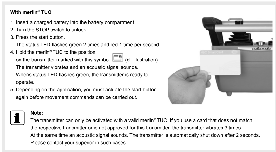
Figure 10. RFID-based user authentication functionality as described in HBC-radiomatic's user manual 25
