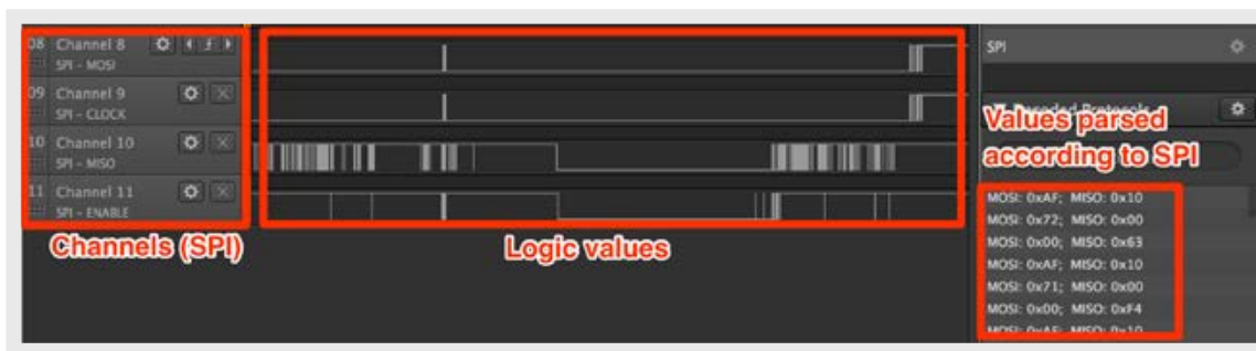
Figure 34. Output of the logic analyzer (bottom right) while tapping on the SPI bus
