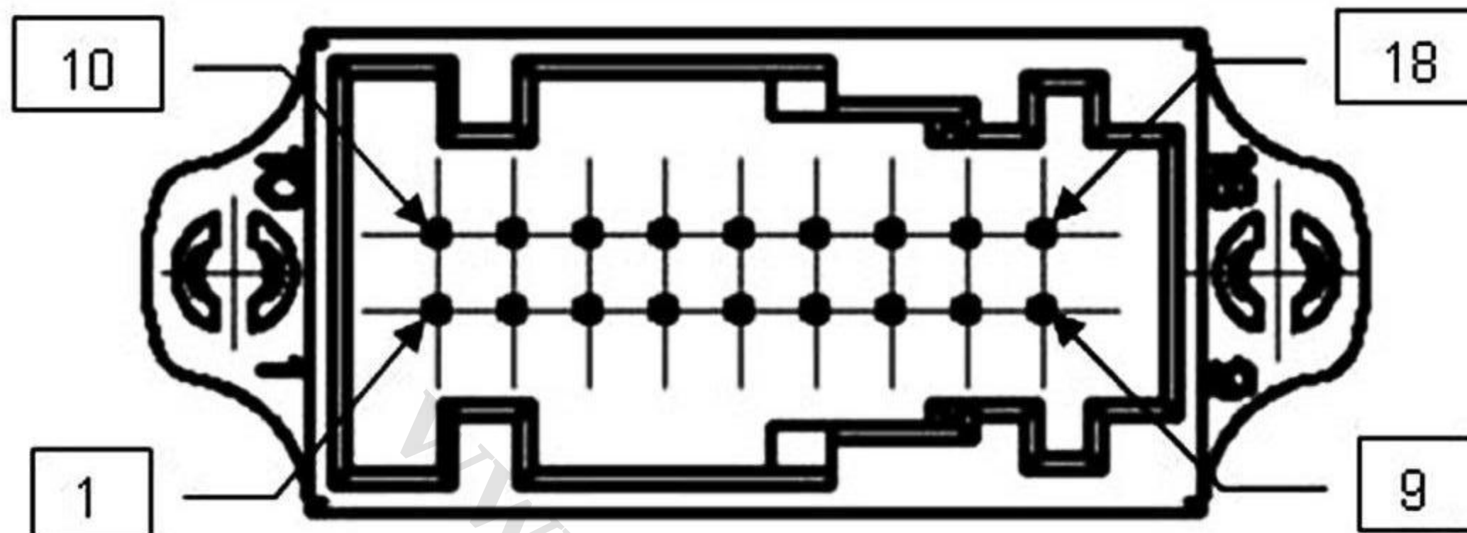
AMP 18PIN VERTICAL CONNECTOR – 953264-1(White)
