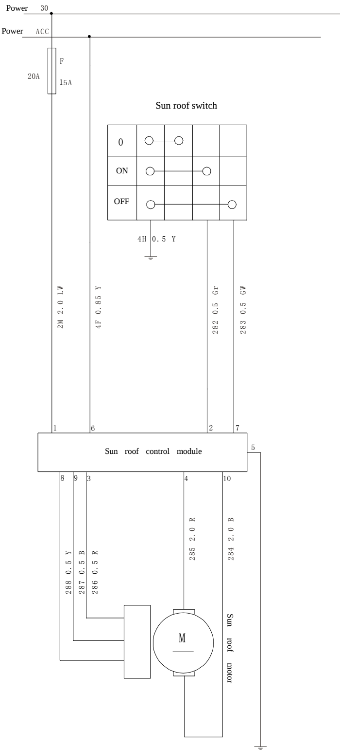
Figure 12-13 Sun roof system schematic diagram
