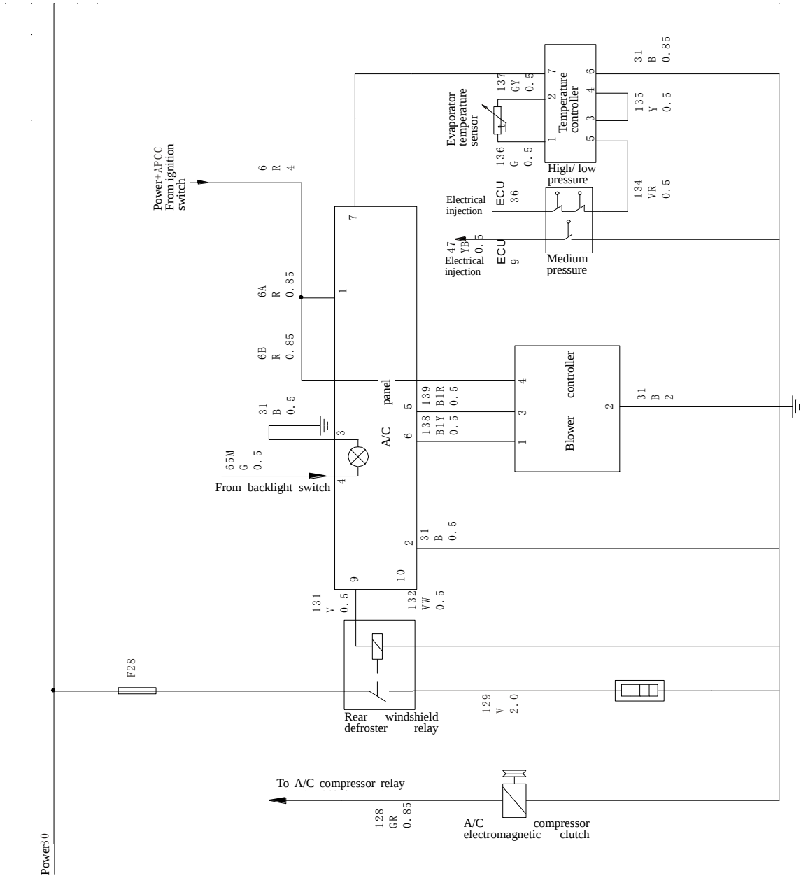
Figure 12-10 Air conditioner system schematic diagram
