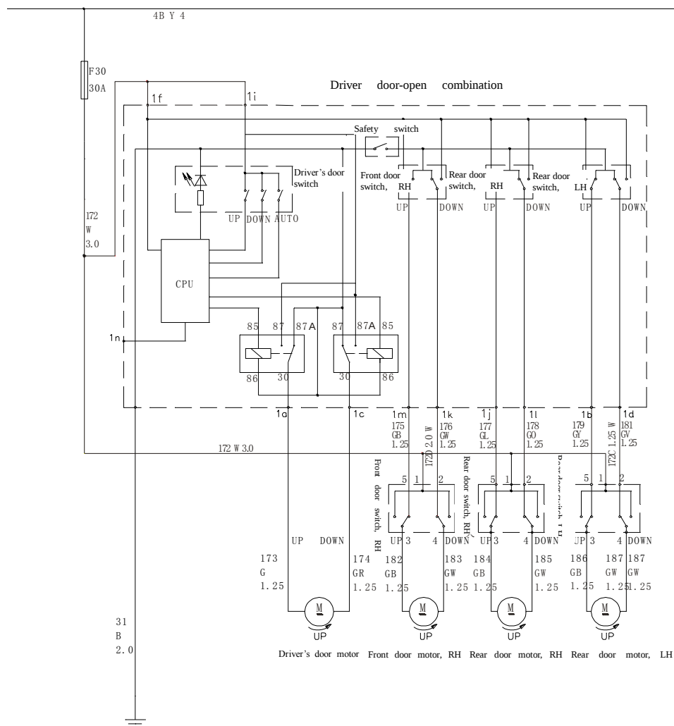
Figure 12-14 Window lifter schematic diagram
