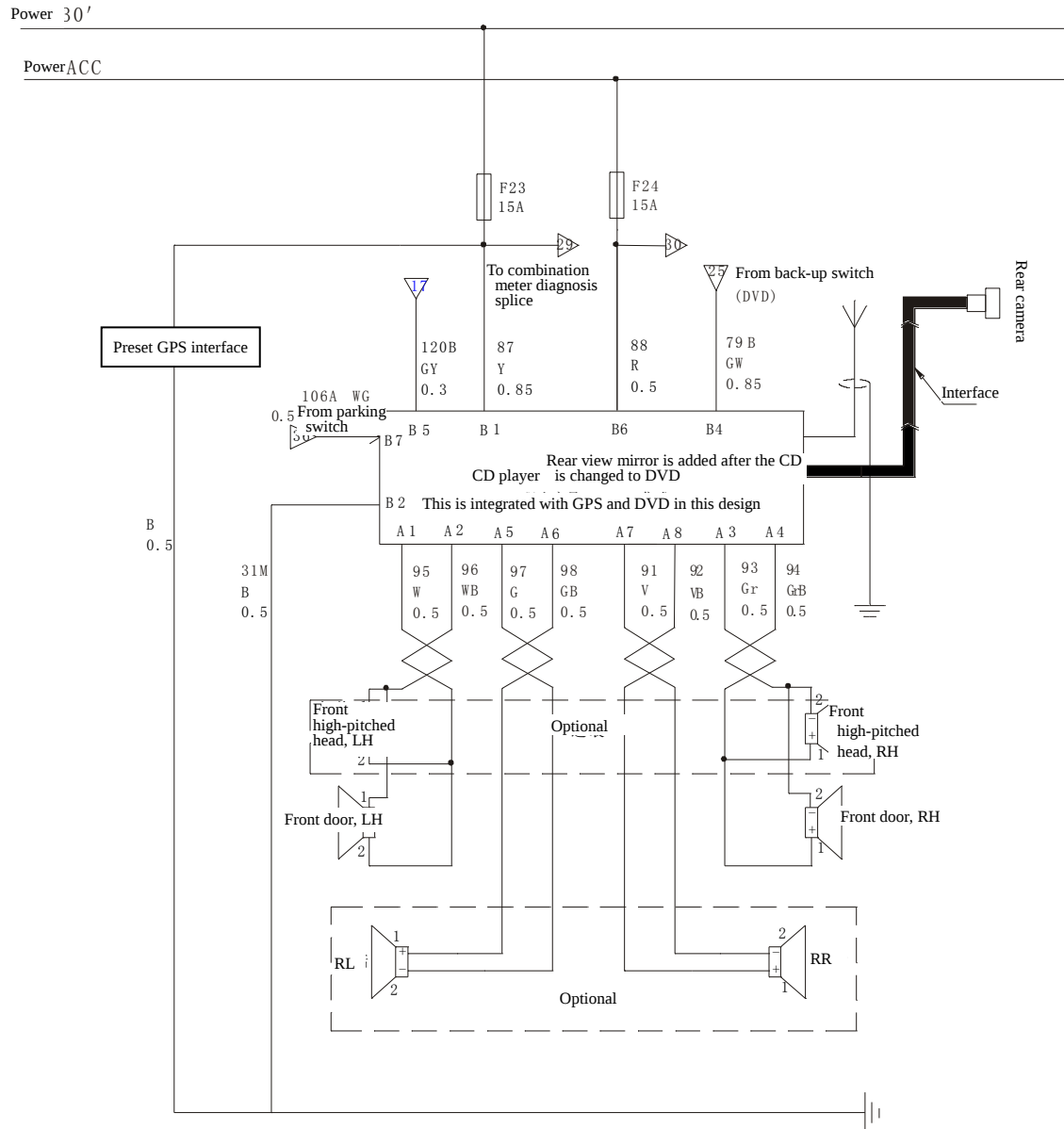
Figure 12-7 Audio system schematic diagram
