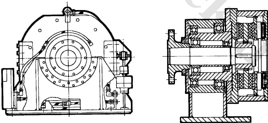
Figure 8.12 Water-cooled friction brake used as a dynamometer
