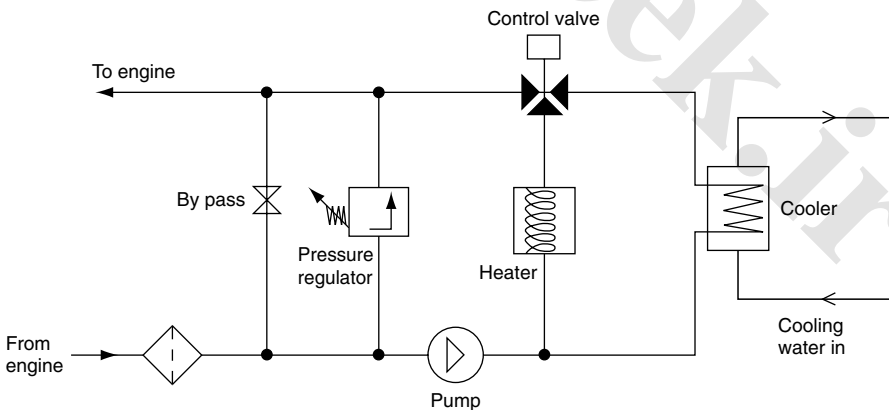
Figure 7.7 Schematic of oil temperature control unit with sensing points and control connections omitted
