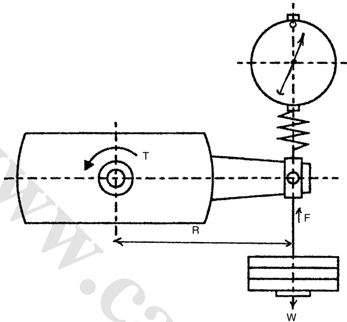
Figure 8.1 Diagram of Froude type, trunnion-mounted, sluice-gate dynamometer measuring torque with dead weights and spring balance
