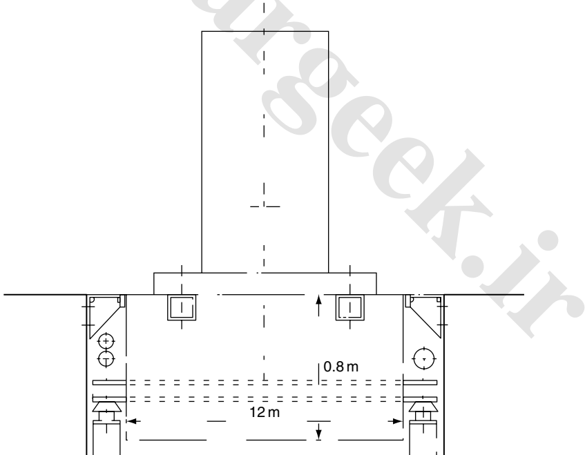
Figure 3.8 Spring-mounted seismic block
