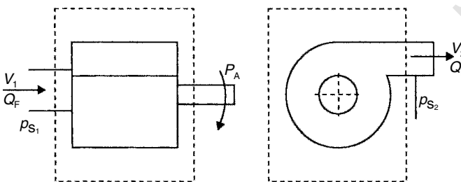
Figure 5.8 Centrifugal fans as an open system
