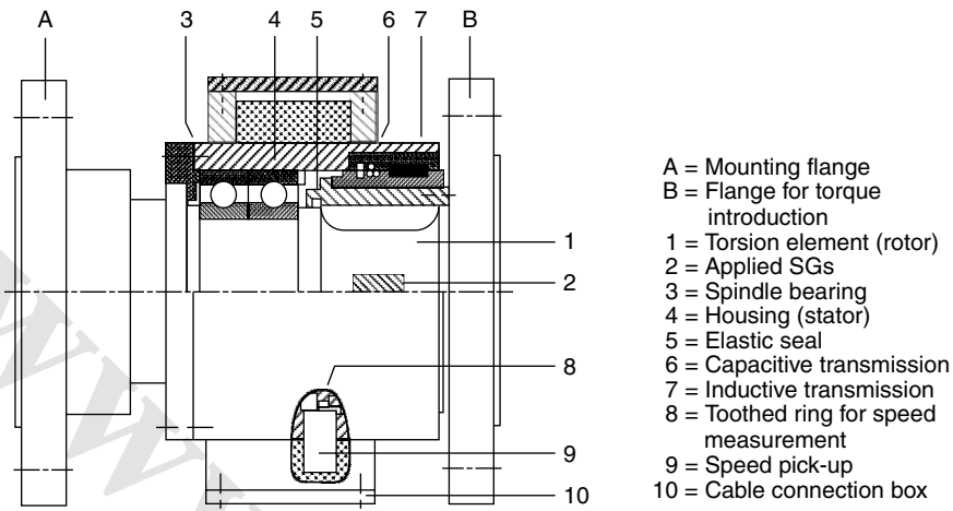
Figure 8.4 Brushless torque-shaft for mounting in shaft-line between engine and 'brake'
