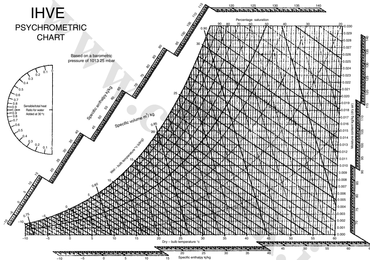
Figure 5.10 Psychrometric chart
