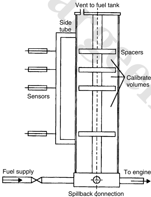
Figure 12.1 Volumetric fuel consumption gauge
