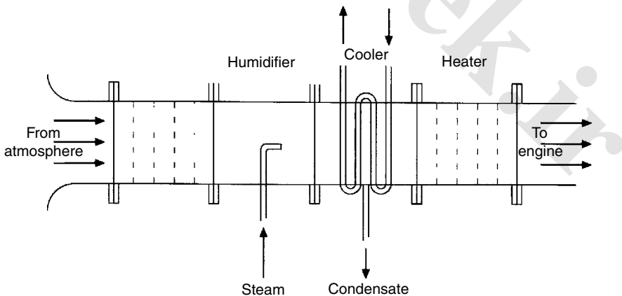
Figure 5.11 Schematic of typical combustion air system contents
