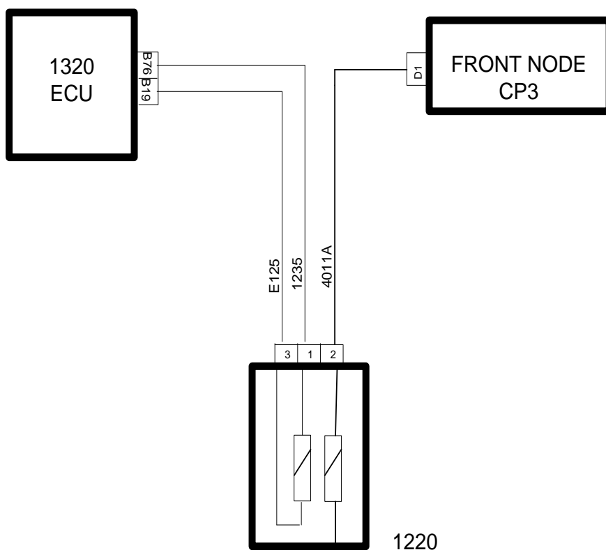
Eng. Coolant Temperature sensor
